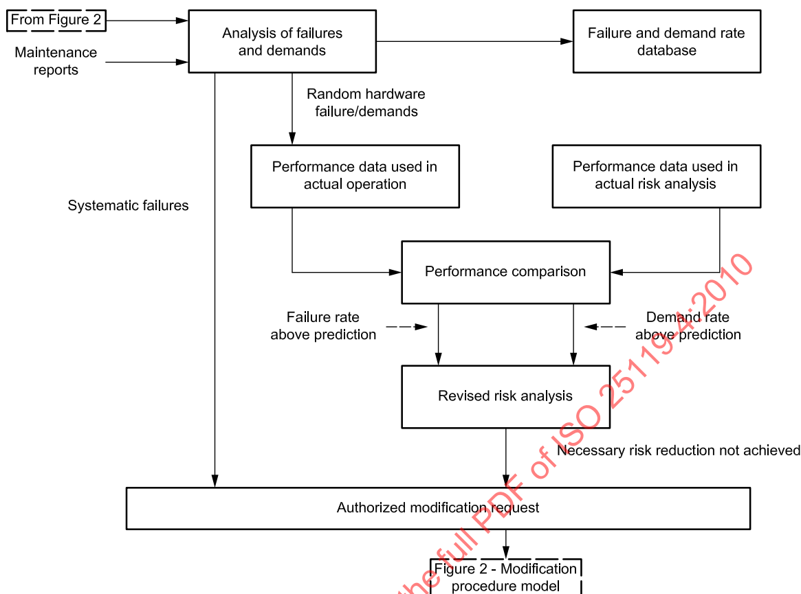
Figure 3 — Example operation and maintenance management model
