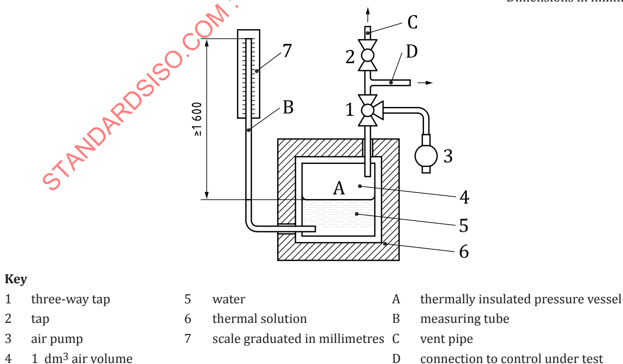
Figure B.1 — Leak-tightness test apparatus (pressure-loss method)
