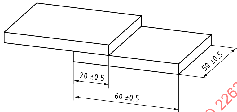
Figure 3 — Shear test specimen
