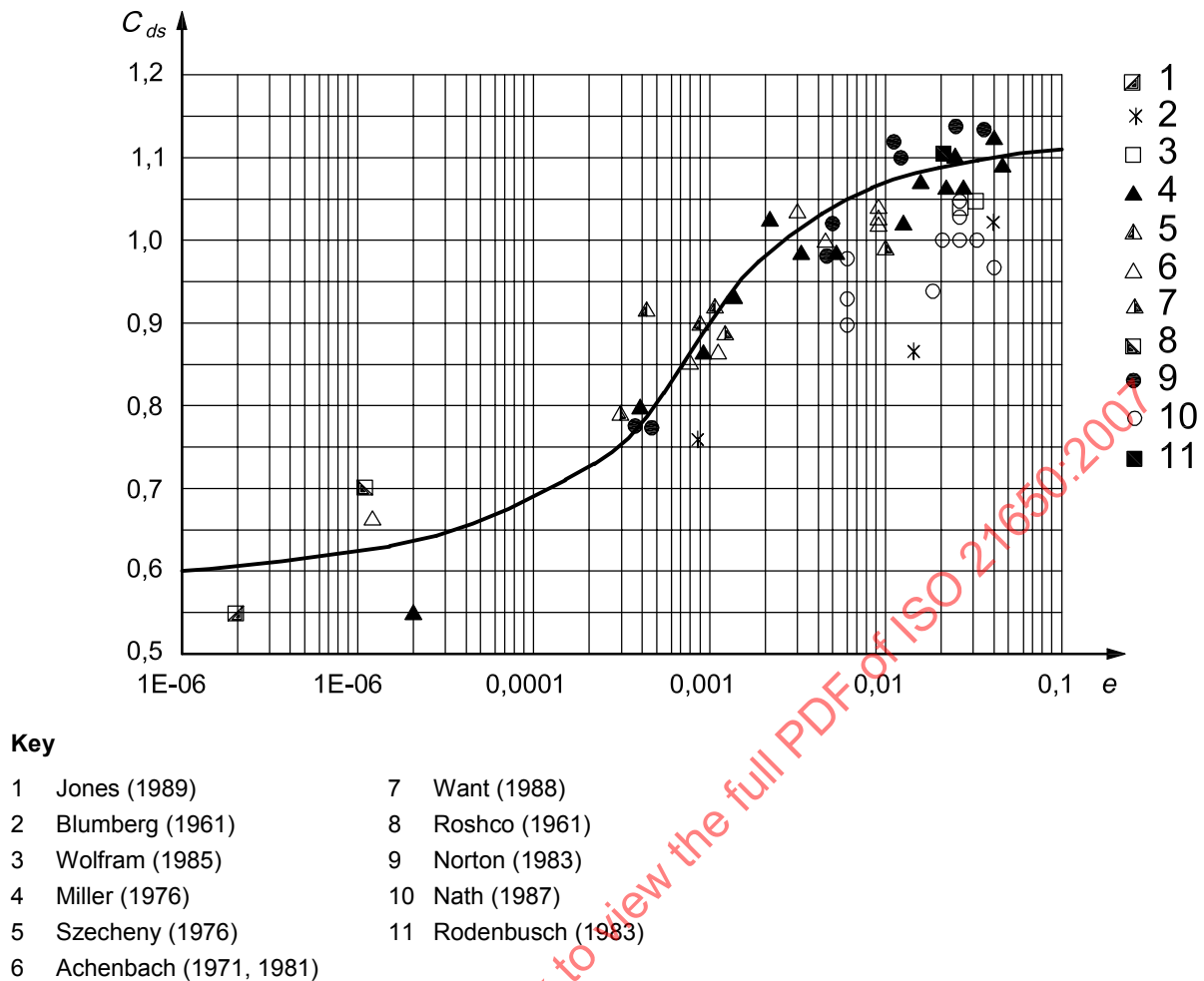
Figure G.1 — Dependence of steady flow drag coefficient for circular cylinders on relative surface roughness (See ISO 19902 [115] )
