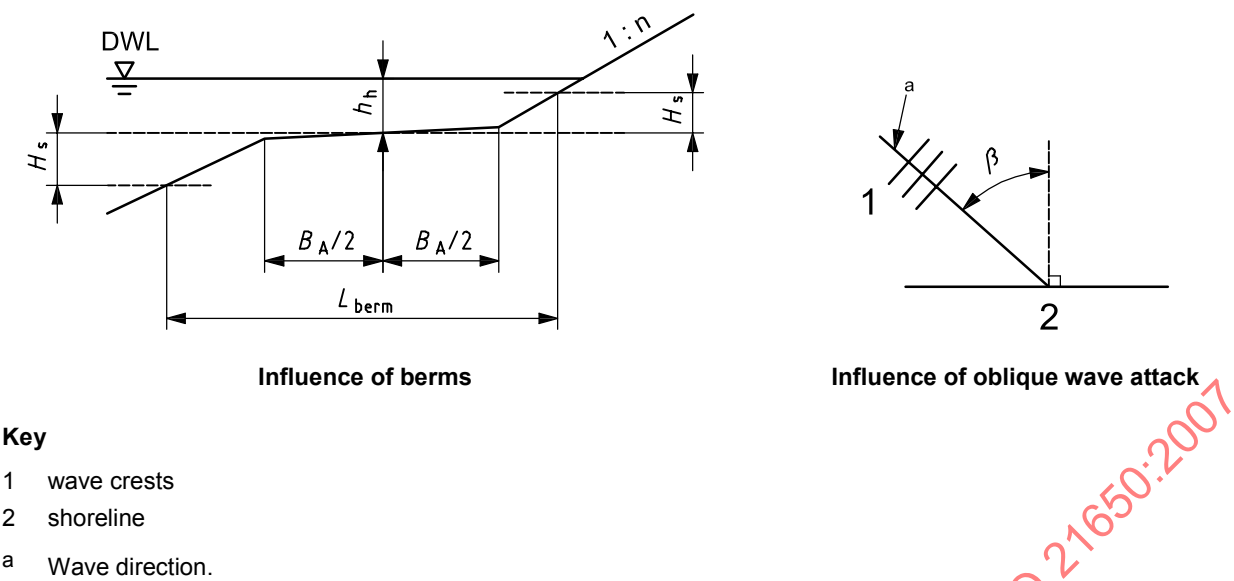
Figure F.2 — Reduction coefficients accounting for angle of wave attack and berm influence
