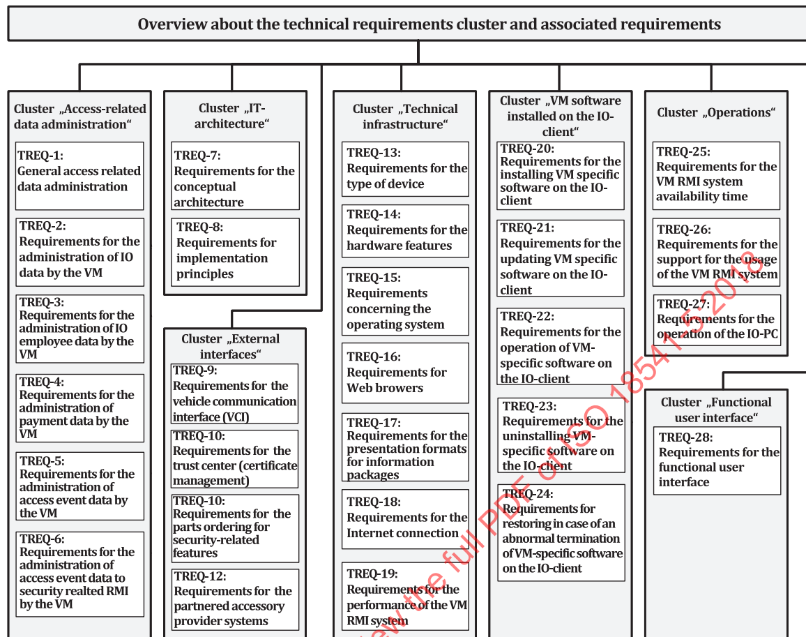
Figure 4 — Overview about the technical requirements clusters
