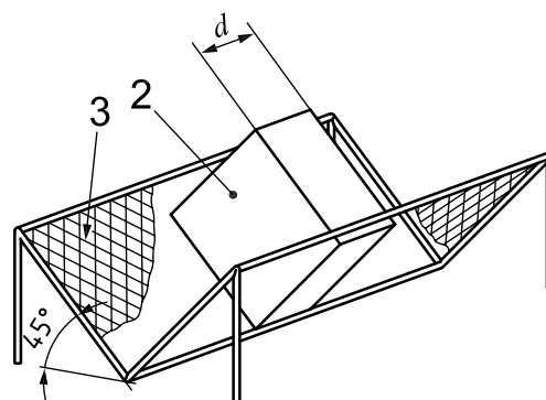
Figure 3 — Example of equipment for the determination of water absorption by total immersion (Method 2C)
