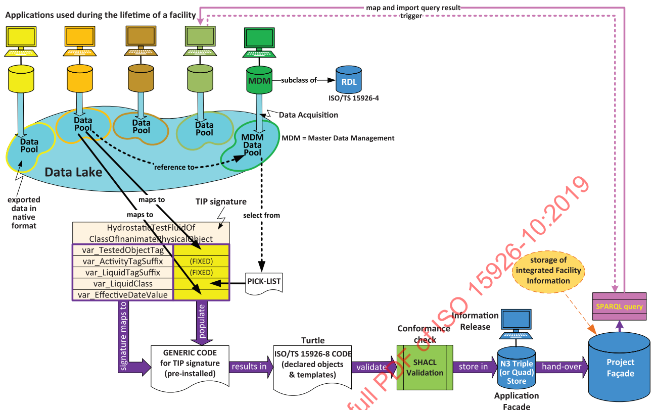
Figure 12 — Overview of activities
