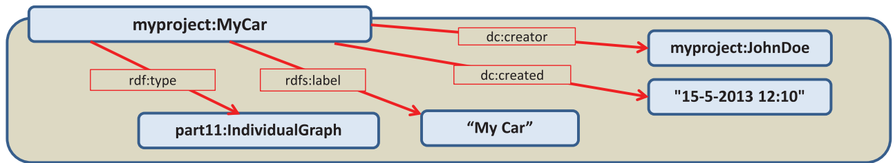
Figure D.3 — Example of an individual graph: RDF Named Graph introducing a placeholder with the label “MyCar”
