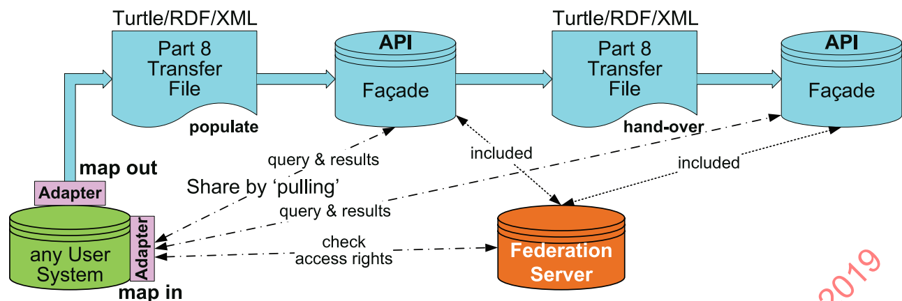
Figure 11 — Information integration
