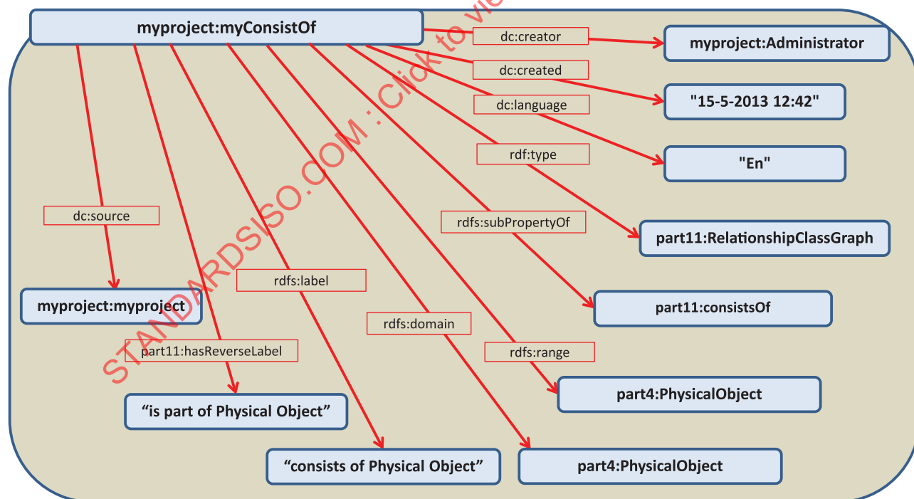
Figure D.2 — Example of a relationship graph: RDF Named Graph introducing a specialized relationship from part11:consistsOf
