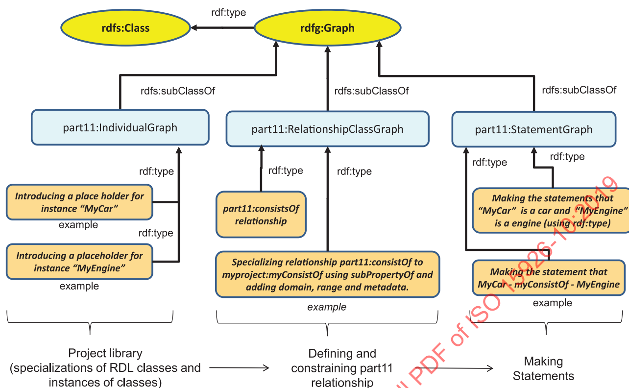
Figure D.1 — Three kinds of Named Graphs: individual graph, relationship graph, and statement graph
