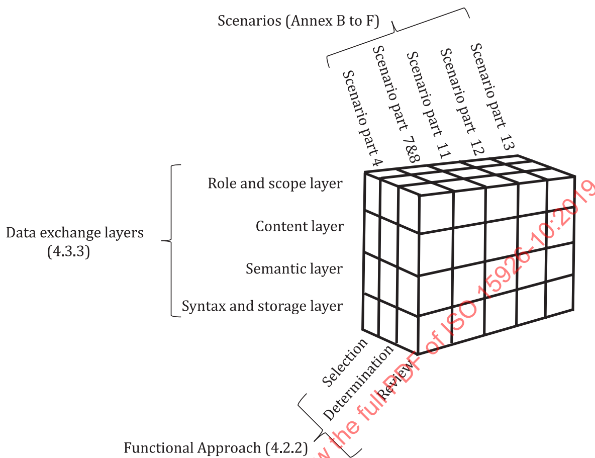
Figure 8 — Combining data exchange layers with conformance steps
