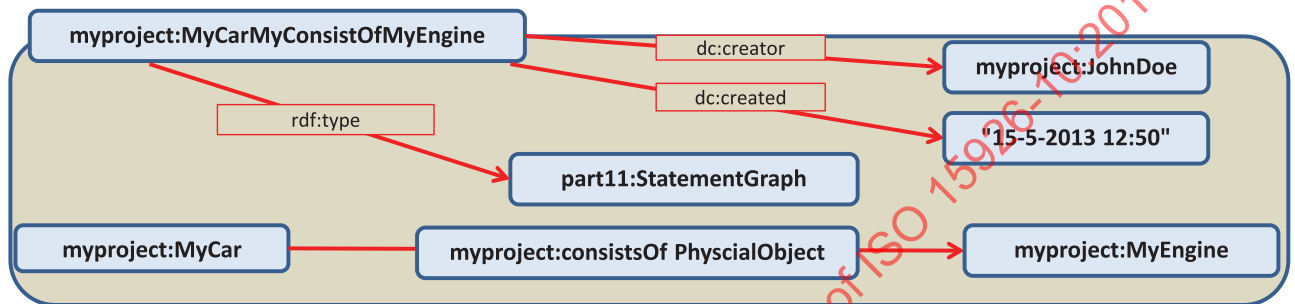
Figure D.4 — Example of a statement graph: RDF Named Graph stating that “MyCar consistsOfPhysicalObject of MyEngine”
