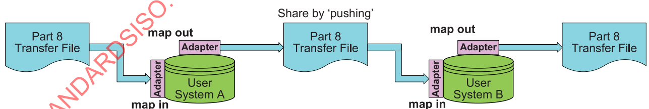
Figure 10 — Application-to-application interfacing
