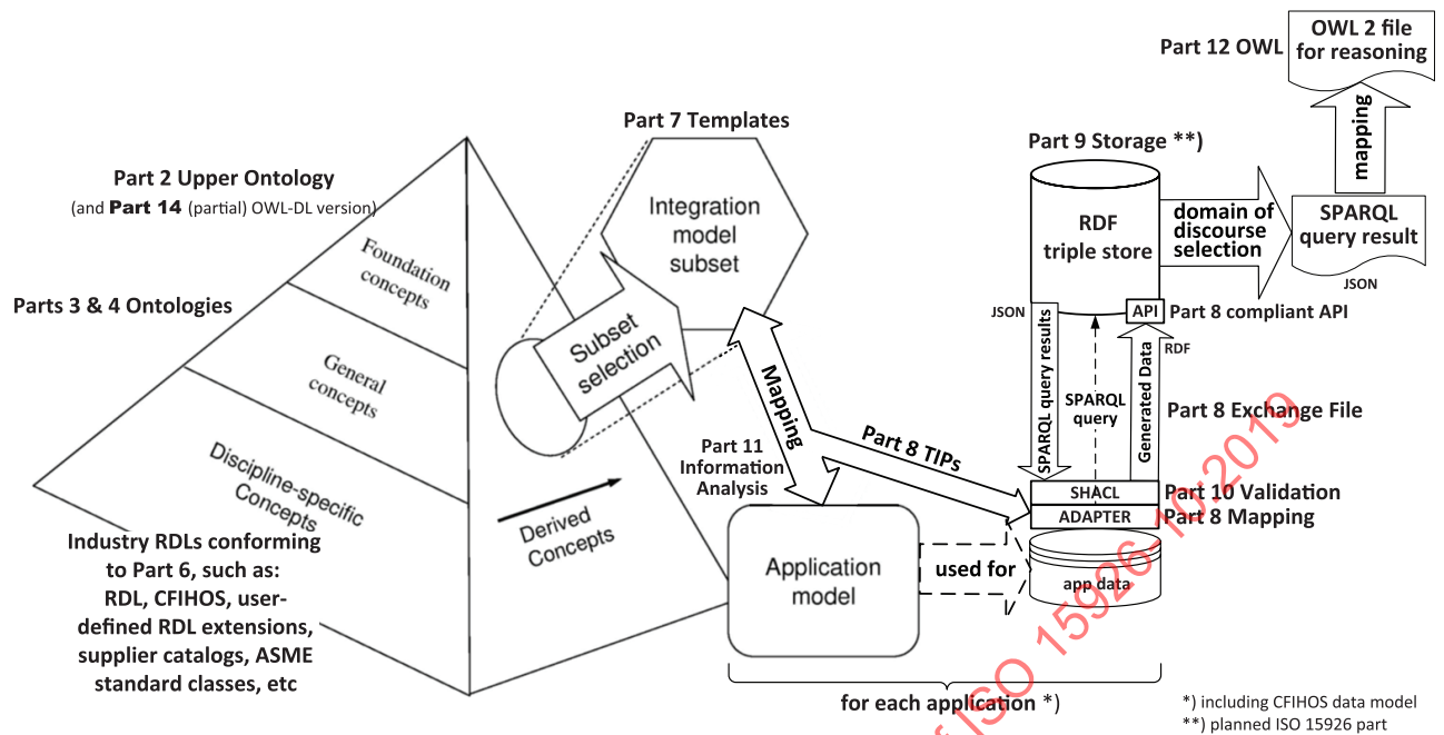
Figure 9 — Overview of the integration architecture of ISO 15926
