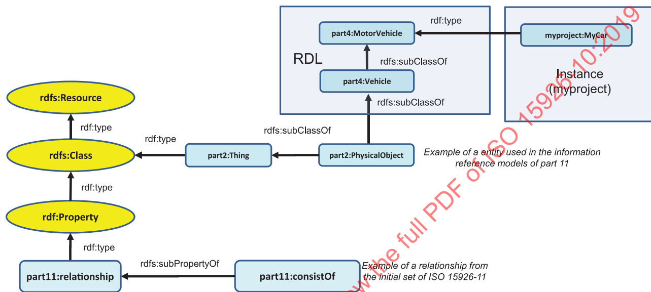
Figure 13 — Connection of ISO/TS 15926-11 with RDF “resource”
