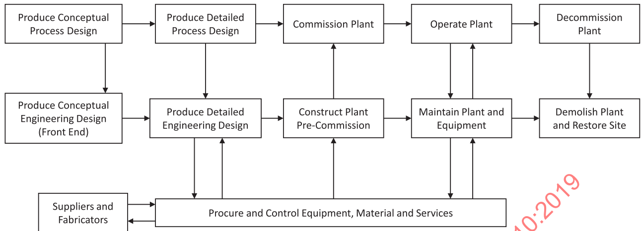
Figure 1 — ISO 15926-1 activity model
