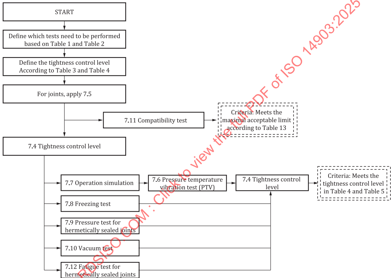
Figure 2 — Test procedure
