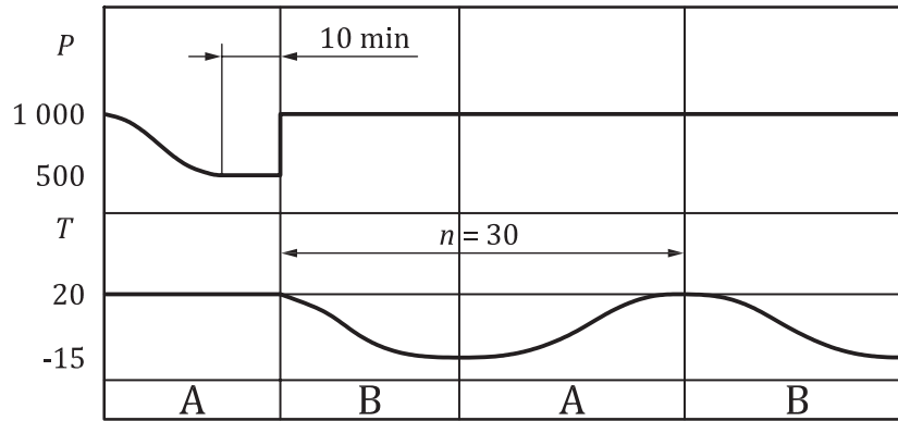
a) Pressure and temperature during the freezing test
