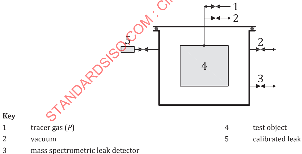
Figure 3 — Principle of tightness control — Tracer gas
