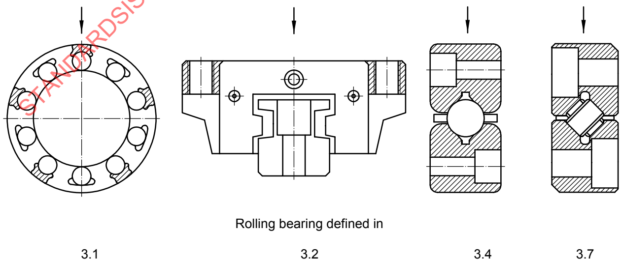
Figure 8 — Direction of load
