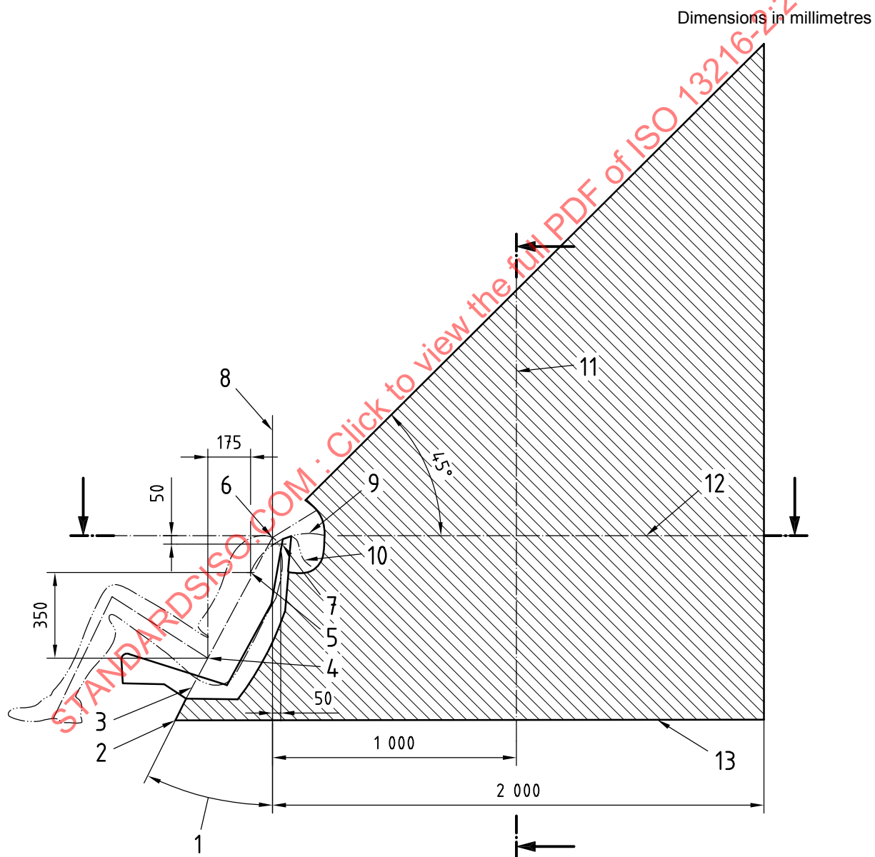
Figure 2 — Top tether anchorage location — ISOFIX zone — Side view
