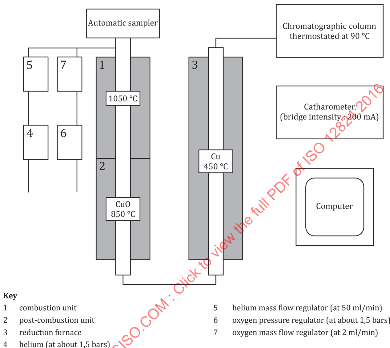
Figure C.2 — Elemental analyser unit
