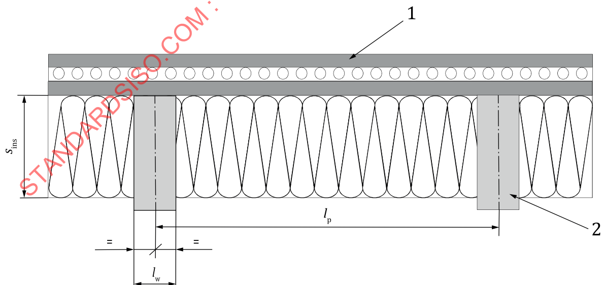
Figure 4 — Effective thickness and effective thermal conductivity of thermal insulating layer of profiled thermal insulating panel — Type B
