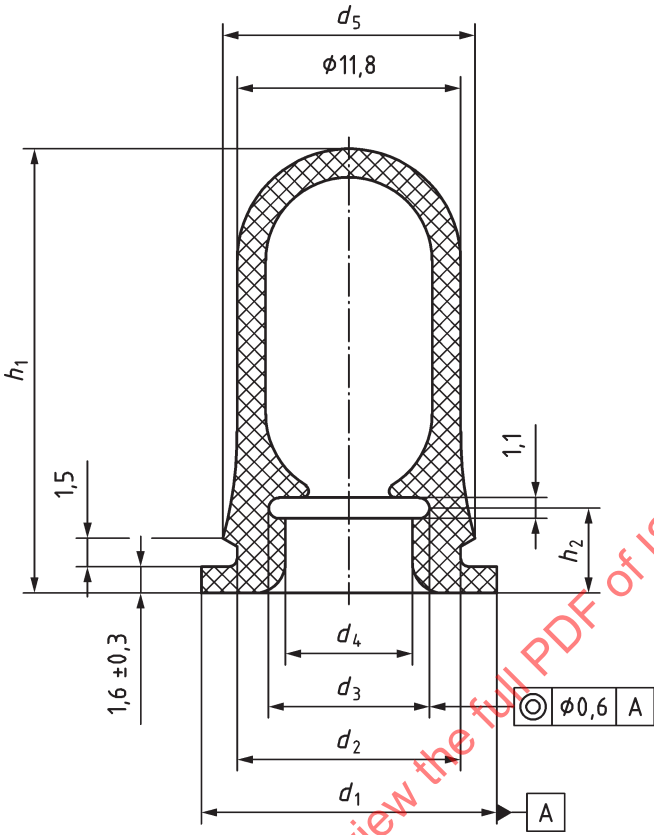
Figure 3 — Dropper bulb with medium suction volume
