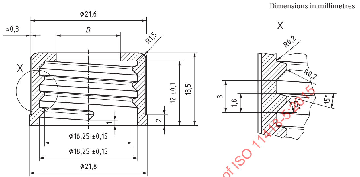
Figure 4 — Screw cap
