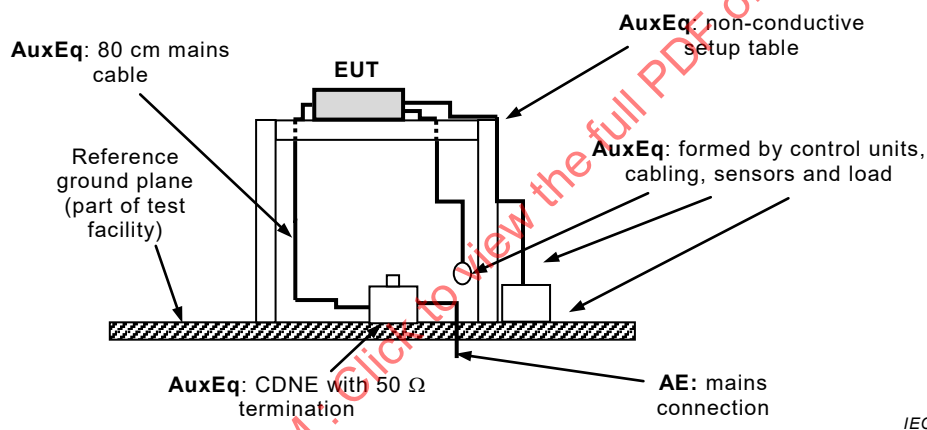
Figure C.5 – Example of arrangement of an external module during the radiated (OATS, SAC or FAR) disturbance measurement
