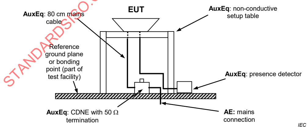
Figure C.3 – Example of arrangement of a luminaire during the radiated (OATS, SAC or FAR) disturbance measurement
