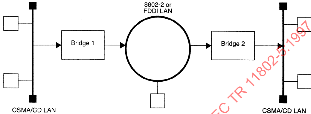
Figure 5—Frame-flow configuration
