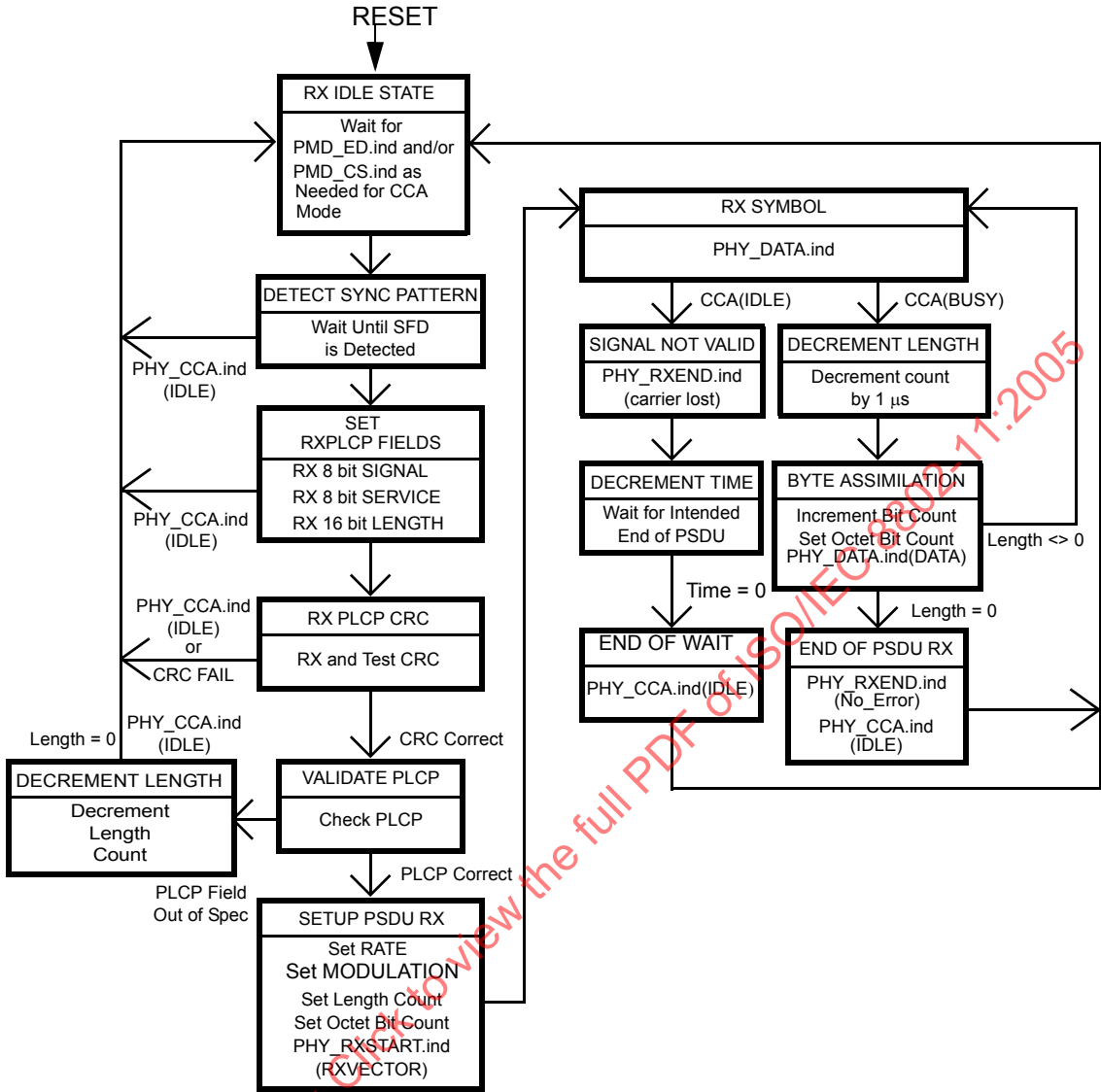
Figure 140—PLCP receive state machine
