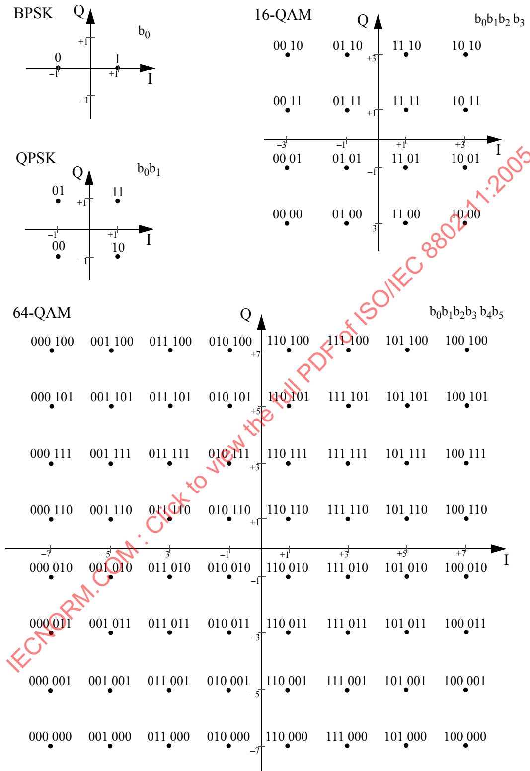
Figure 120—BPSK, QPSK, 16-QAM, and 64-QAM constellation bit encoding
