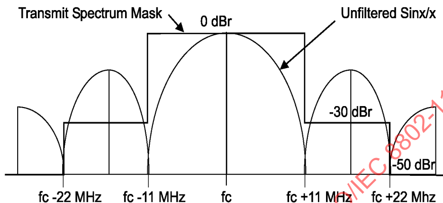
Figure 149—Transmit spectrum mask
