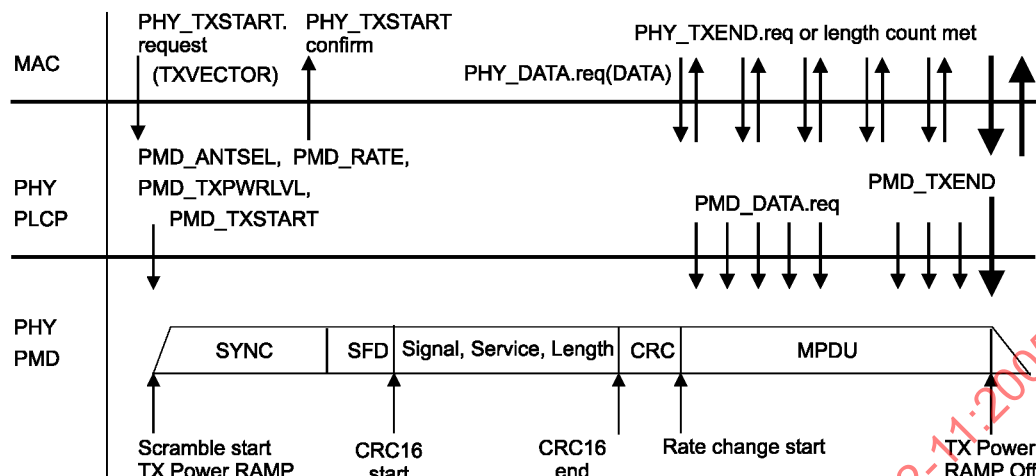
Figure 95—Transmit PLCP
