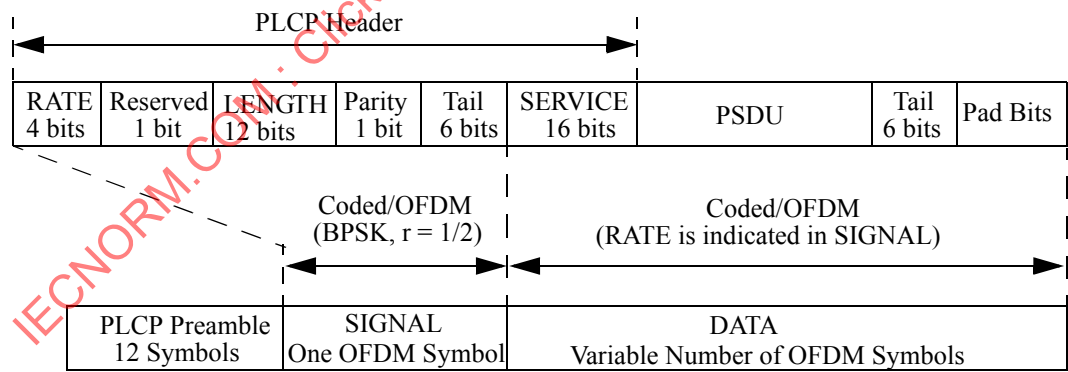
Figure 111—PPDU frame format
