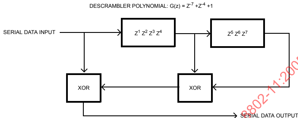
Figure 136—Data descrambler
