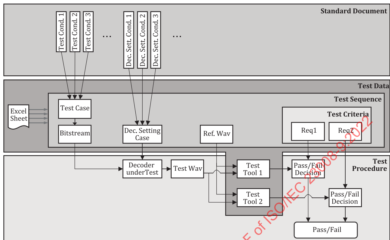
Figure 1 — Conformance testing components
