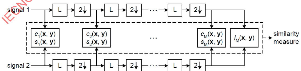
Figure 1 — MS-SSIM calculation procedure
