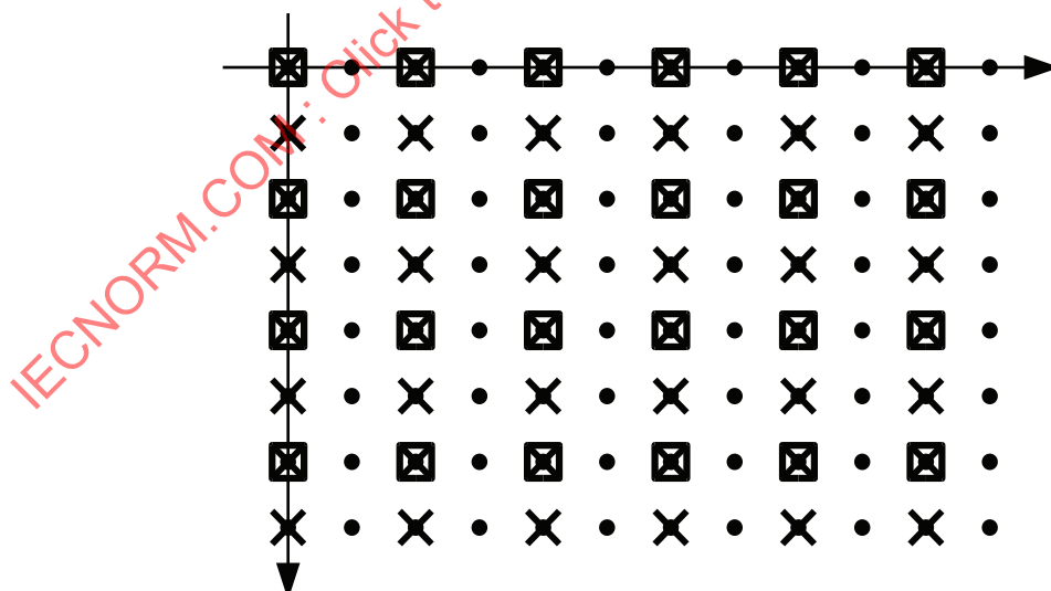
Figure B.1 — Sampling grid for 4:2:2 sampling
