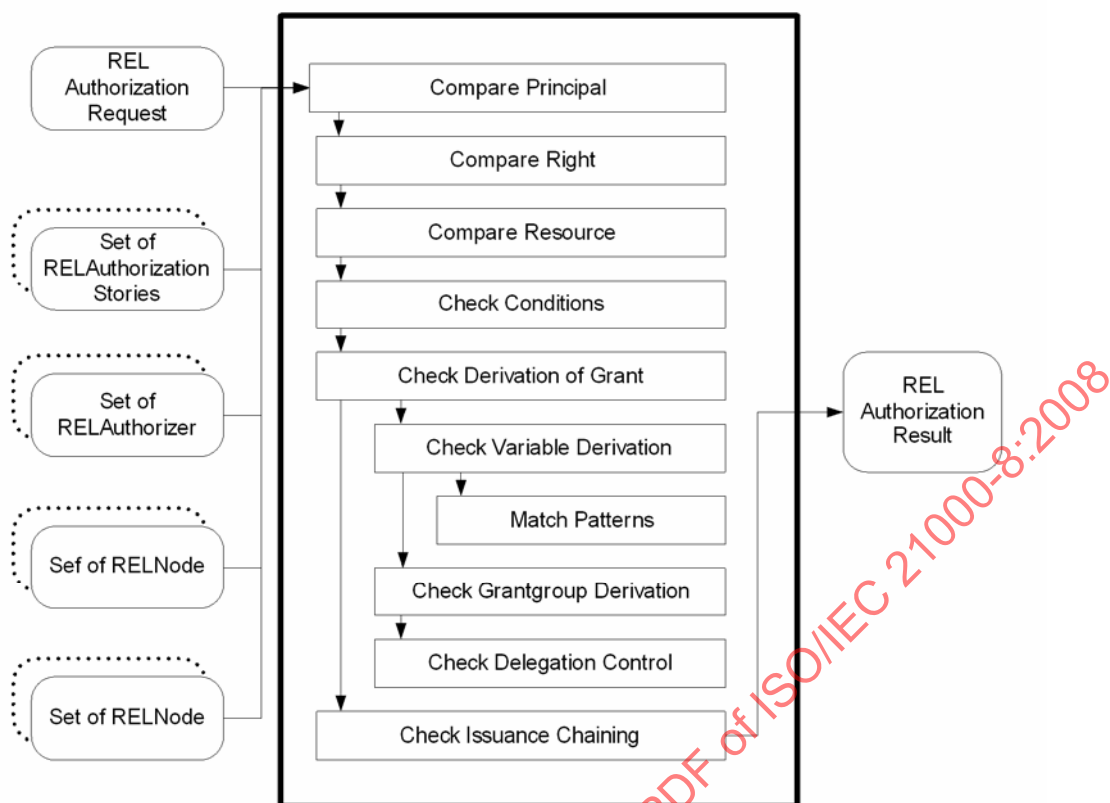
Figure 8 — REL Interpretation Reference Software Architecture Diagram
