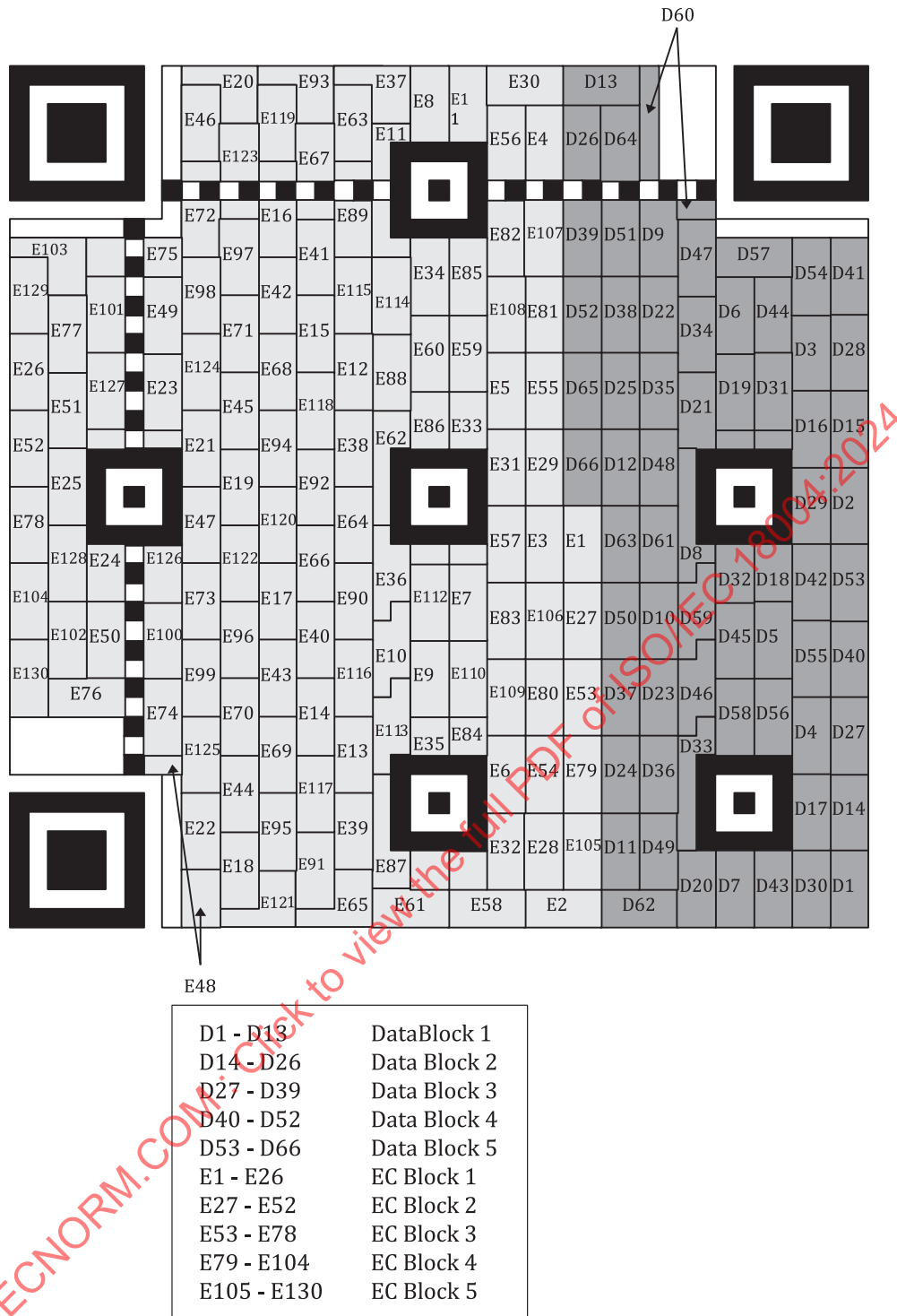
Figure 20 — Symbol character arrangement in a version 7-H symbol
