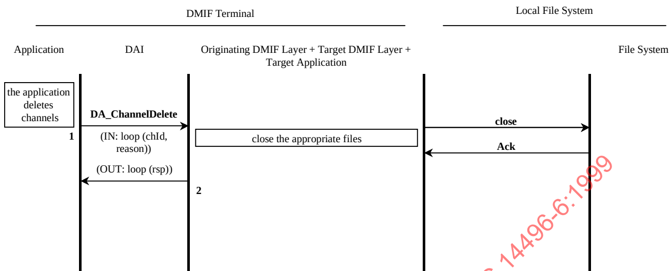
Figure B.12 — Deletion of Channels in a Local Storage DMIF
