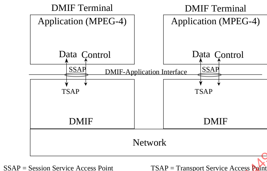
Figure 7 — Position of the DMIF-Application Interface in the DMIF architecture
