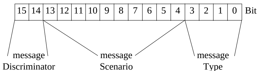
Figure 9 — Format of DMIF Signalling messageId
