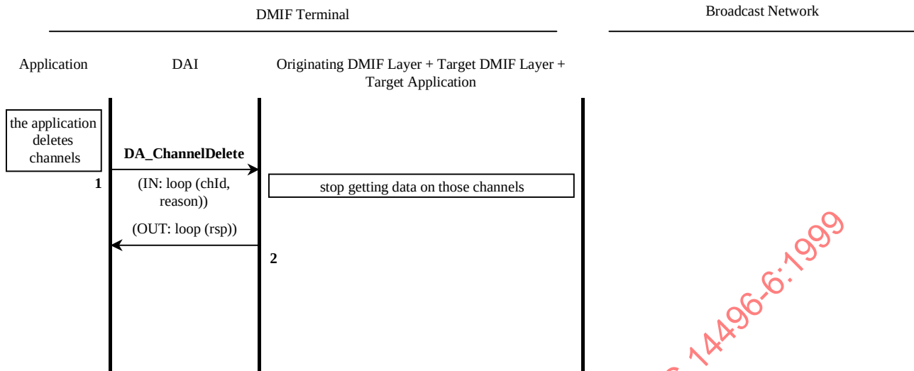
Figure B.8 — Deletion of Channels in a Broadcast DMIF
