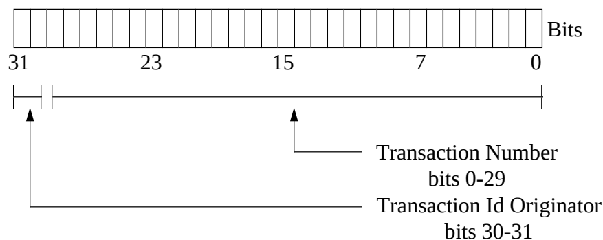
Figure 8 — Format of transactionId field
