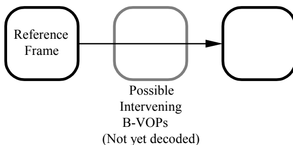
Figure AMD1-24 -- Frame-prediction for P-VOPs
