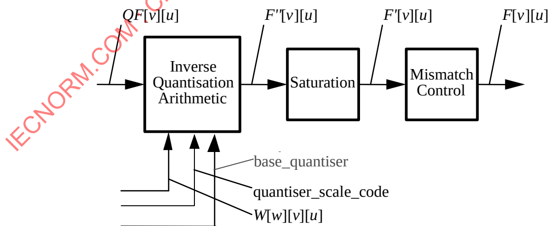
Figure AMD1-15 -- Inverse quantisation process
