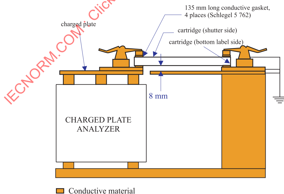
Figure E.1 — Cartridge electro-static discharge test fixture
