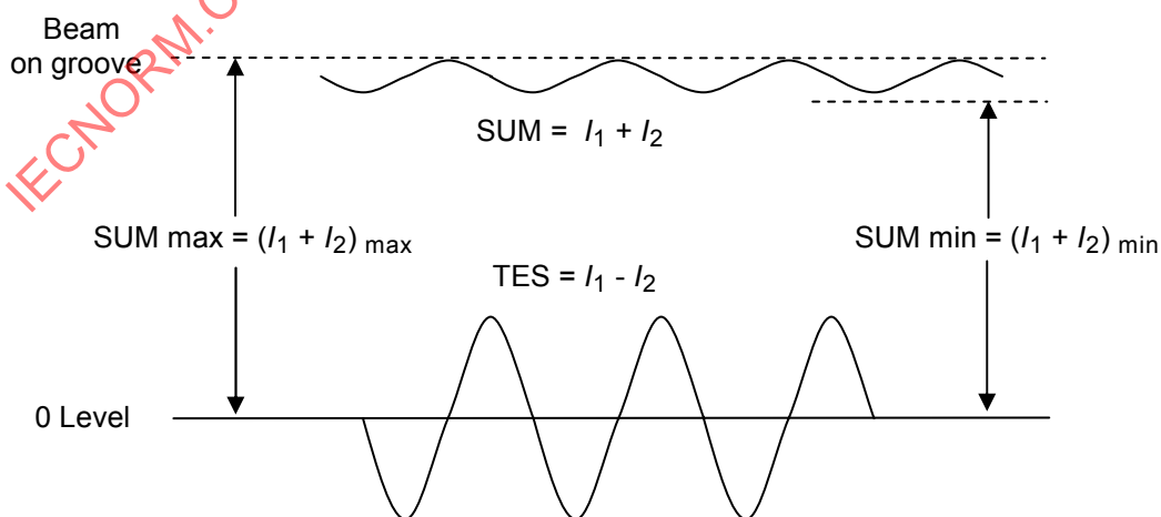
Figure 24 — Signals from grooves in the Radial Tracking Channel
