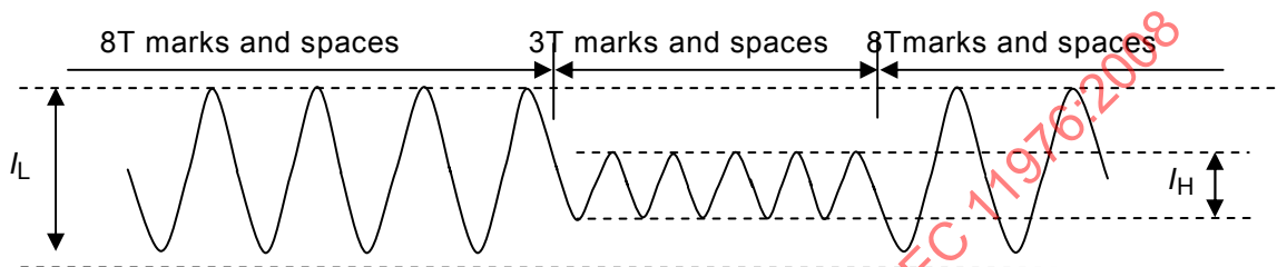
Figure 25 — Definition of I_L and I_H for resolution measurement
