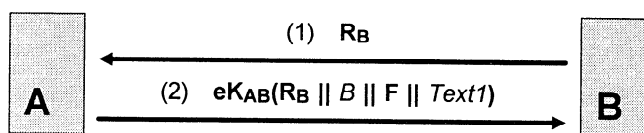
Figure 4 - Mechanism 4
