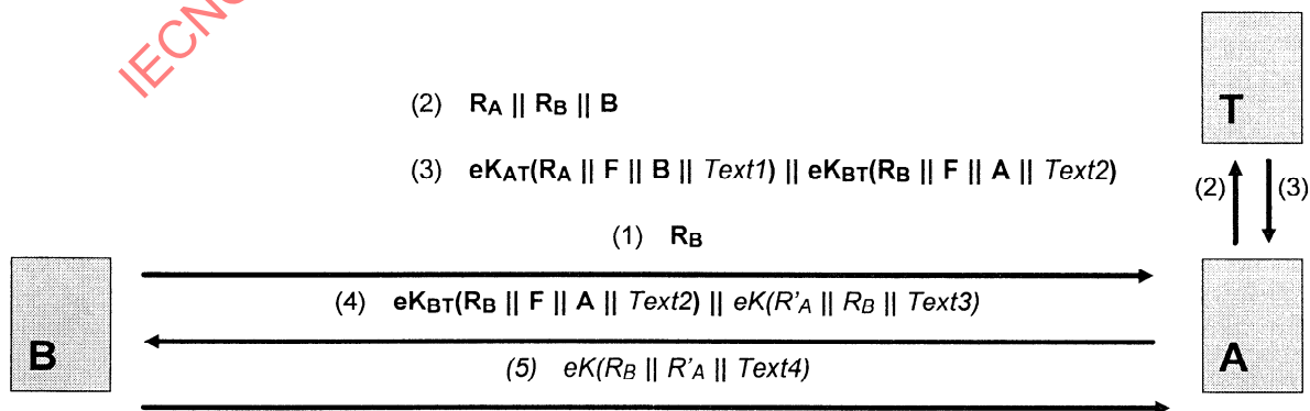
Figure 9 - Mechanism 9
