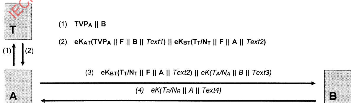
Figure 8 - Mechanism 8
