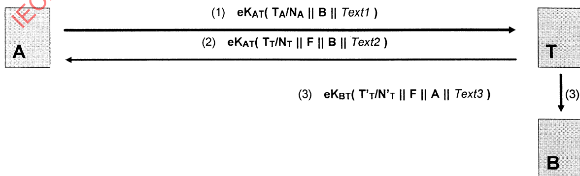
Figure 10 - Mechanism 10
