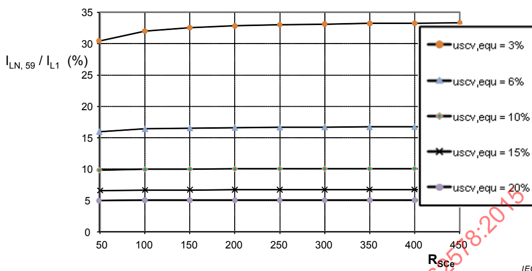
Figure 13 – Basic characteristic of the relative current emission (59th harmonic) of one AIC at a pulse frequency of 3 kHz versus R_{sc} with the line impedance according to 5.2.4
