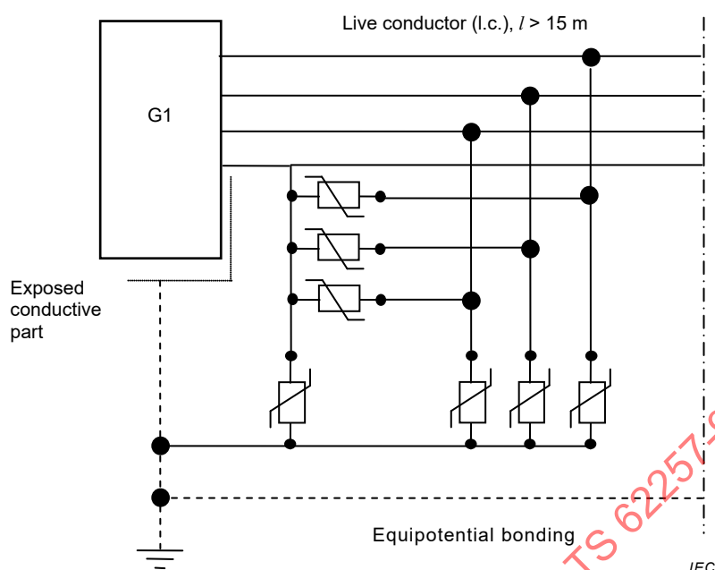
Figure 6 – Example of protection against effects of lightning over-voltage for three phase generators with four live a.c. conductors (TNS P+N scheme) – Generator side
