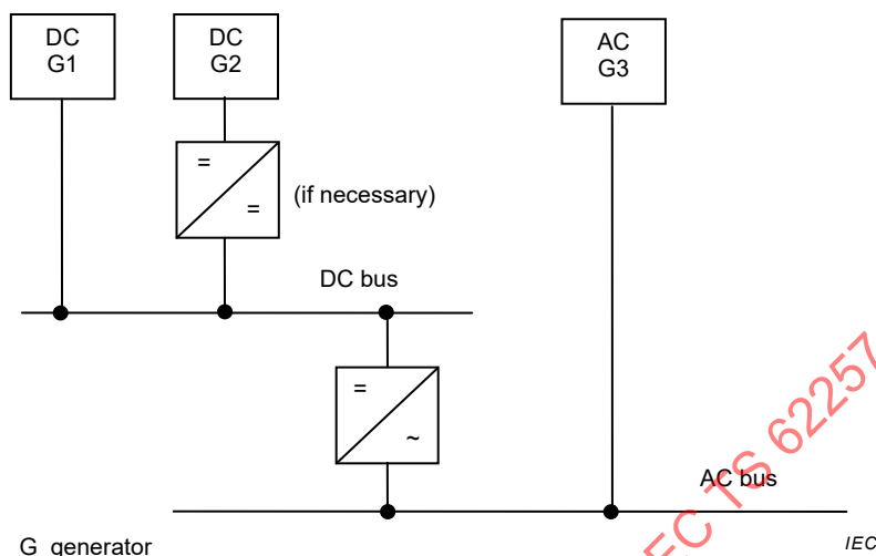
Figure 3 – Interconnection configuration with d.c. bus and a.c. bus
