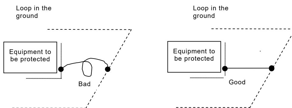
Figure 9 – Wiring arrangement for equipotential link
