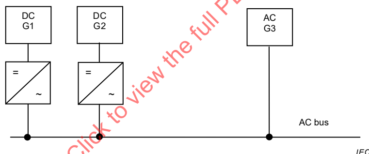
Figure 4 – Interconnection configuration with a.c. bus only
