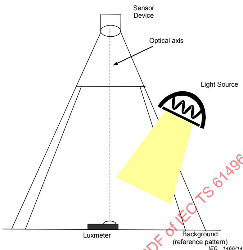
Figure 3 – Light intensity measurement setup for indirect light tests
