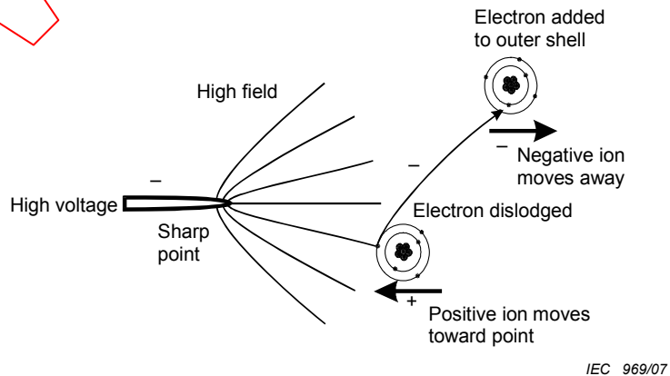
Figure 11 – Corona ionization – Negative
