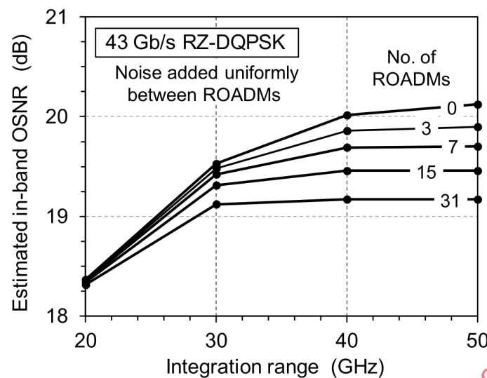
Figure 10 – Impact of integration range on R_{\text{int}} for 43 Gbit/s RZ-DPSK signals in a ROADM network
