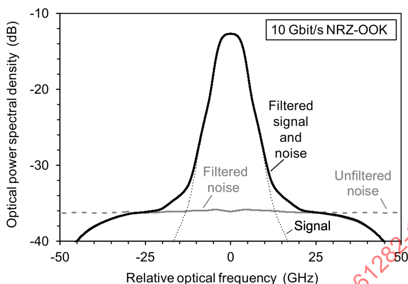
Figure 5 – Power spectral density of a 10 Gbit/s signal with ASE noise that has been shaped by a relatively broad optical filter
