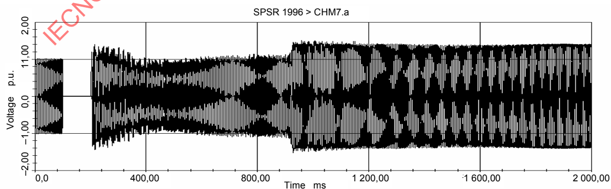
Figure 29 – TOV at LVD7 – Electromagnetic transient simulation with 484 kV switched metal-oxide surge arresters
