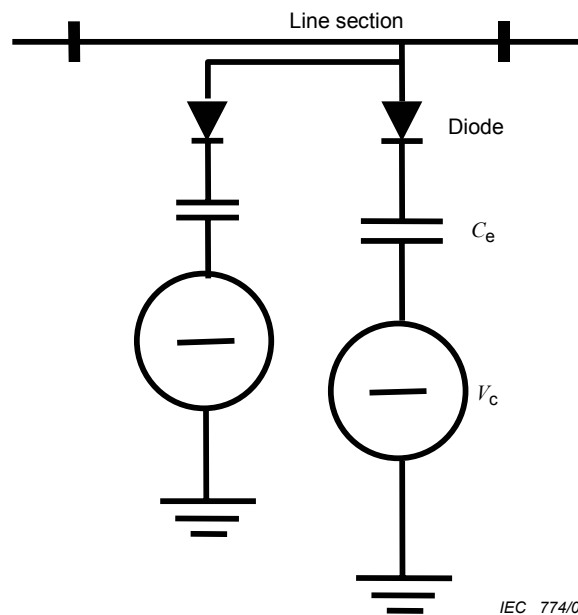
Figure 12 – Example of a corona branch model
