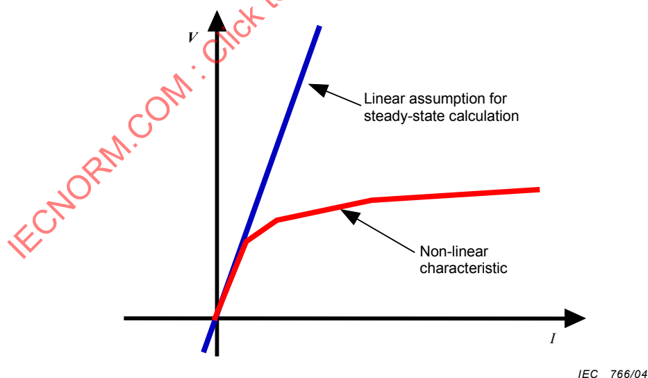
Figure 4 – Example of assumption for the steady-state calculation of a non-linear element
