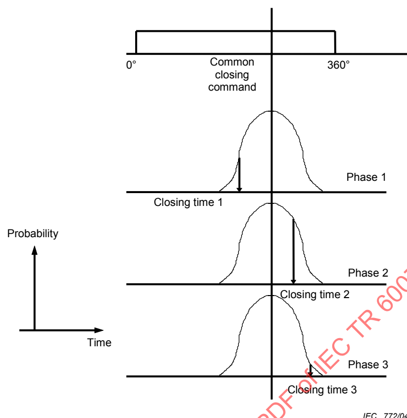
Figure 10 – Diagram showing double distribution used for statistical switches
