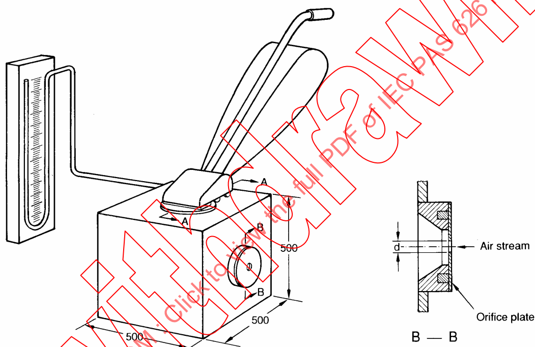
Figure 15c – Alternative B equipment for air data measurements
