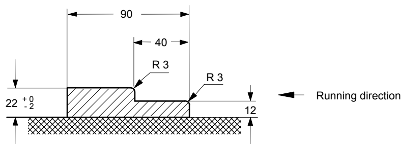
Figure 8a – Profile of threshold
