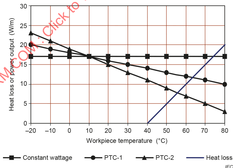
Figure 4 – Equilibrium conditions for upper limit evaluation
