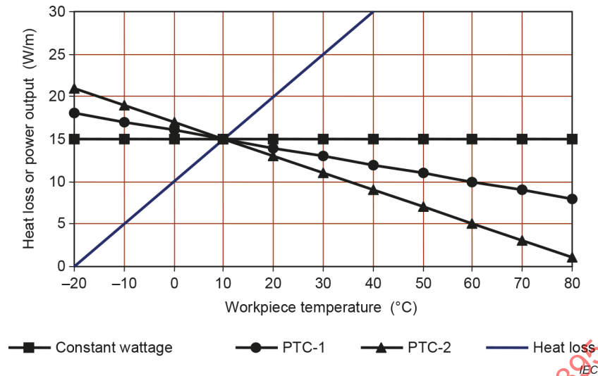
Figure 3 – Equilibrium conditions for workpiece maintenance
