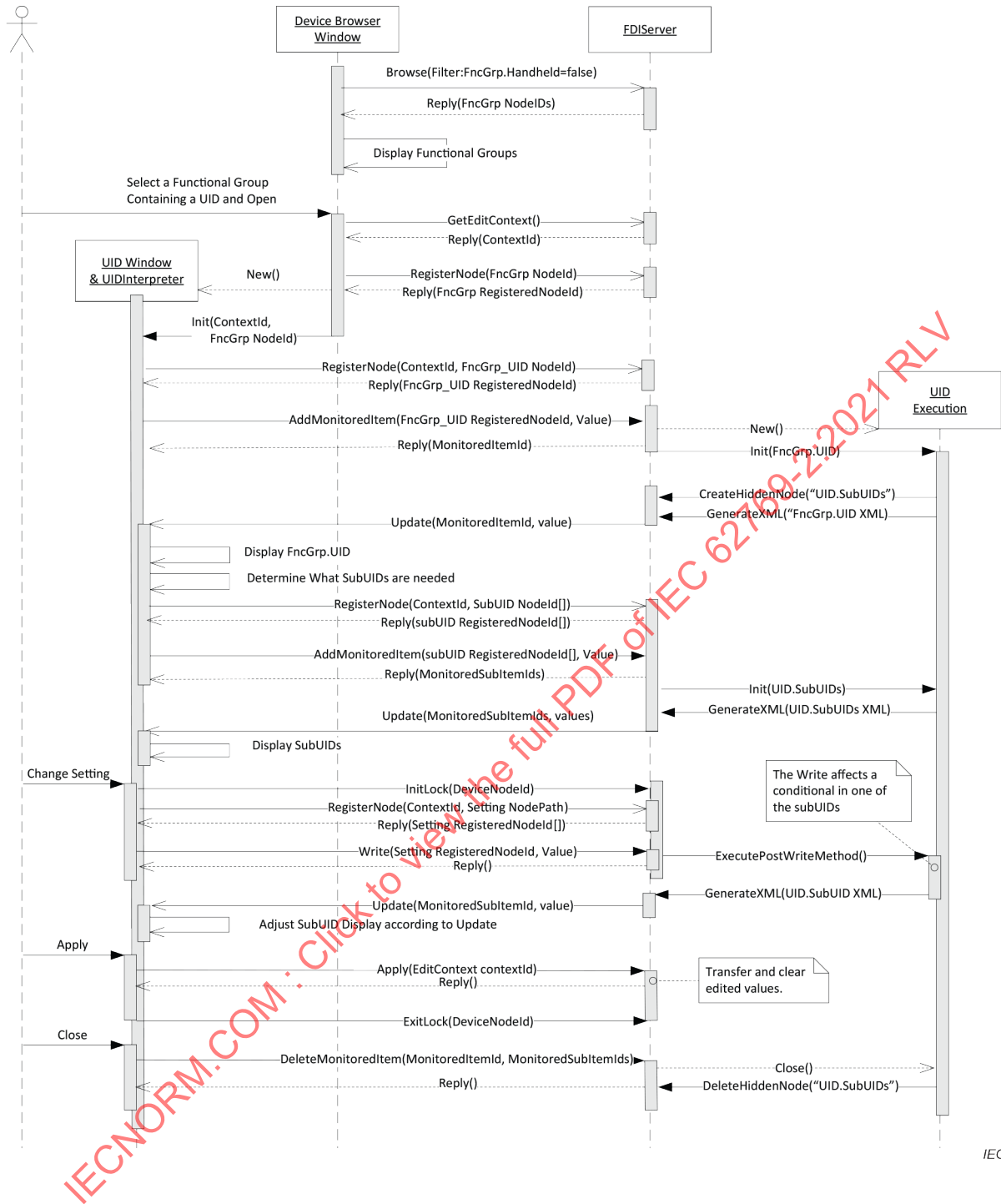
Figure 10 – User Interface Description sequence diagram
