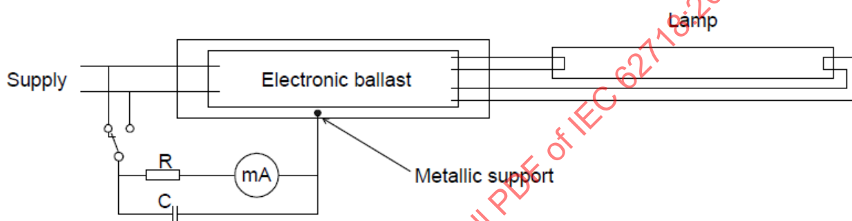
Figure 3 – Circuit for leakage current measurement
