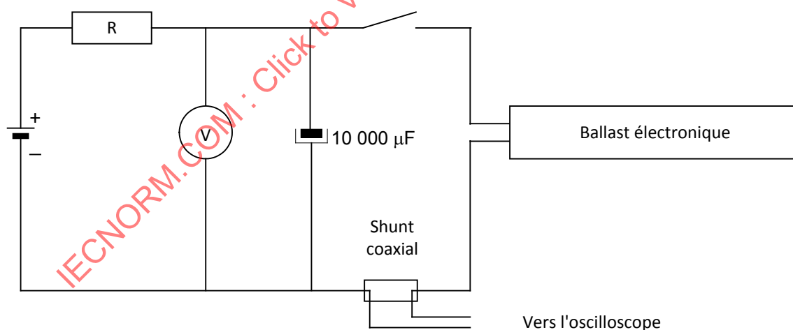
Figure 1 – Circuit d'essai
