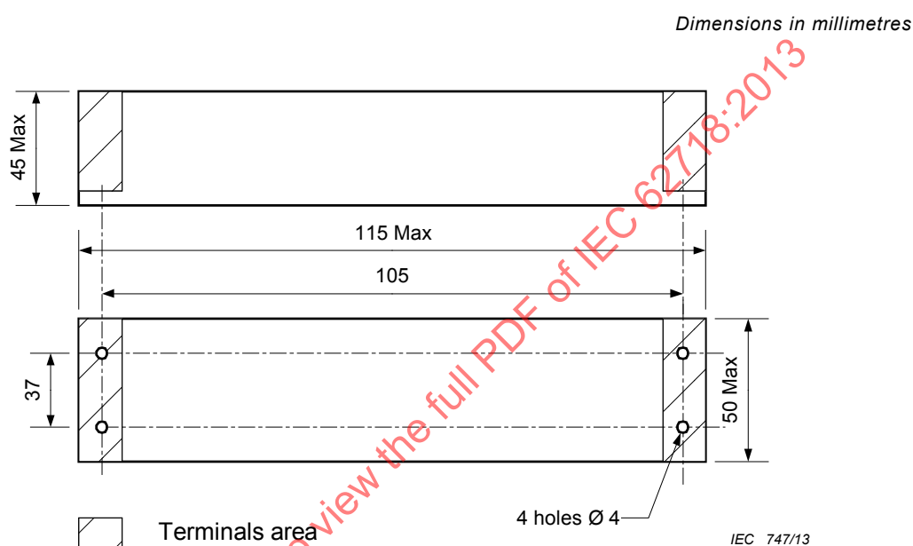
Figure F.1 – Overall dimensions for electronic ballast
