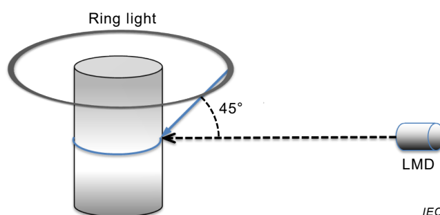
Figure 8 – Example of convex display illuminated by a ring light source
