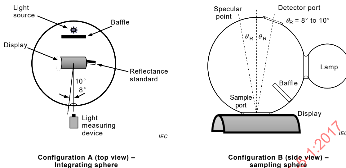
Figure 6 – Example of reflection measurement geometries for spherical illumination
