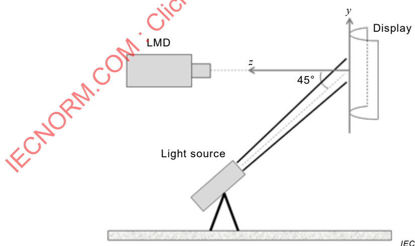
Figure 7 – Example of convex display illuminated by a directed light source
