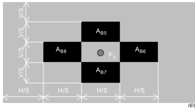
Figure 16 – Cross-talk pattern with perpendicular 4 % black window boxes on grey background
