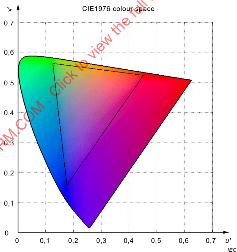
b) CIE 1976 UCS chromaticity diagram
