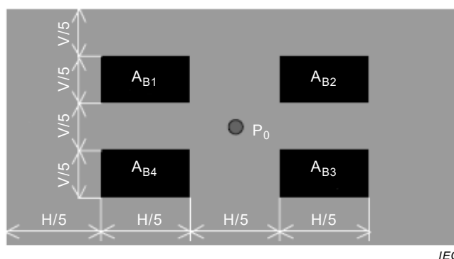
Figure 14 – Cross-talk pattern with diagonal 4 % black window boxes on grey background
