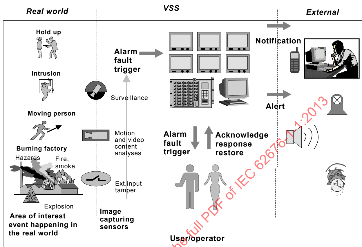
Figure 3 – Activity management
