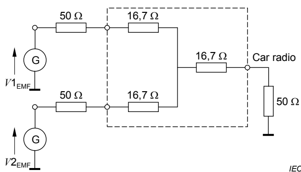
Figure 1 – Coupling circuit
