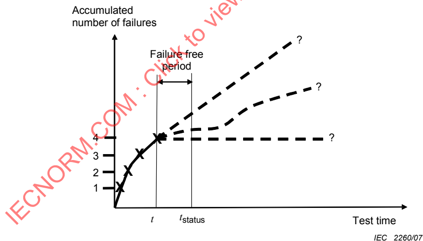
Figure 2 – Evaluating whether the cumulative failure curve has levelled out
