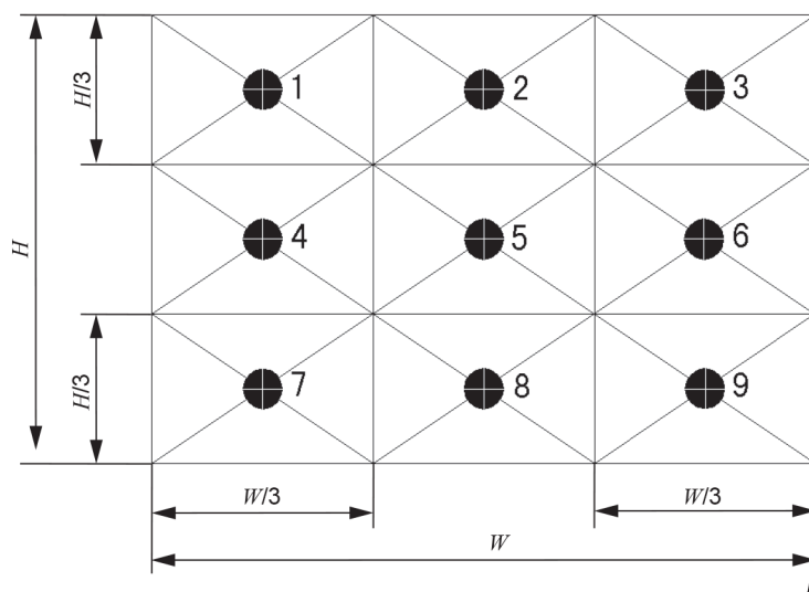
Figure 2 – Standard measurement positions in the display active area
