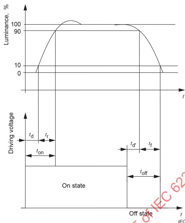
Figure A.1 – Relationship between driving signal and optical response times
