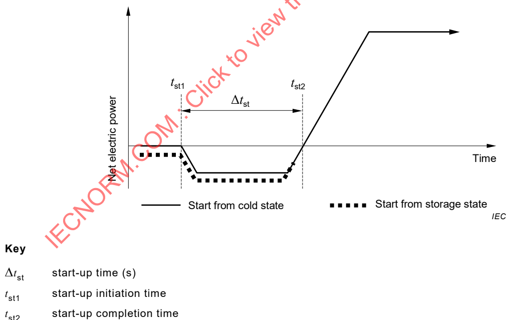
Figure 7 – Example of electric power chart during start-up time for system without battery
