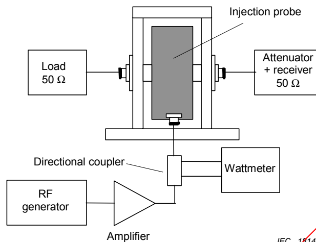
Figure 4 – Calibration set-up
