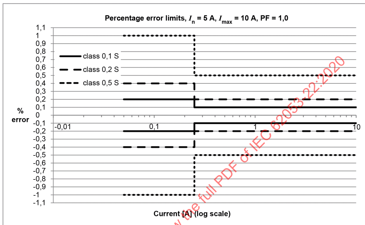
Figure A.1 – Comparison of acceptable percentage error limits for meters of classes 0,1 S, 0,2 S, and 0,5 S, with I_n = 5 \text{ A} and I_{\max} = 10 \text{ A} , at \text{PF} = 1,0
