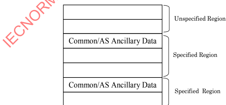
Figure 39 – Generic compound data block structure
