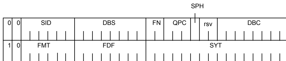
Figure 5 – Common isochronous packet (CIP) format
