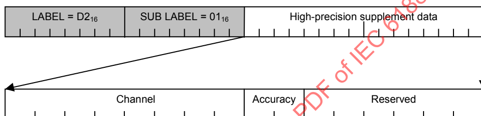
Figure 45 – High-precision first ancillary data
