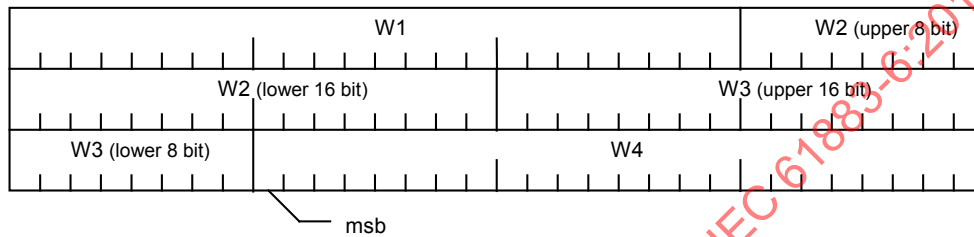
Figure 28 – 24-bit × 4 audio pack format
