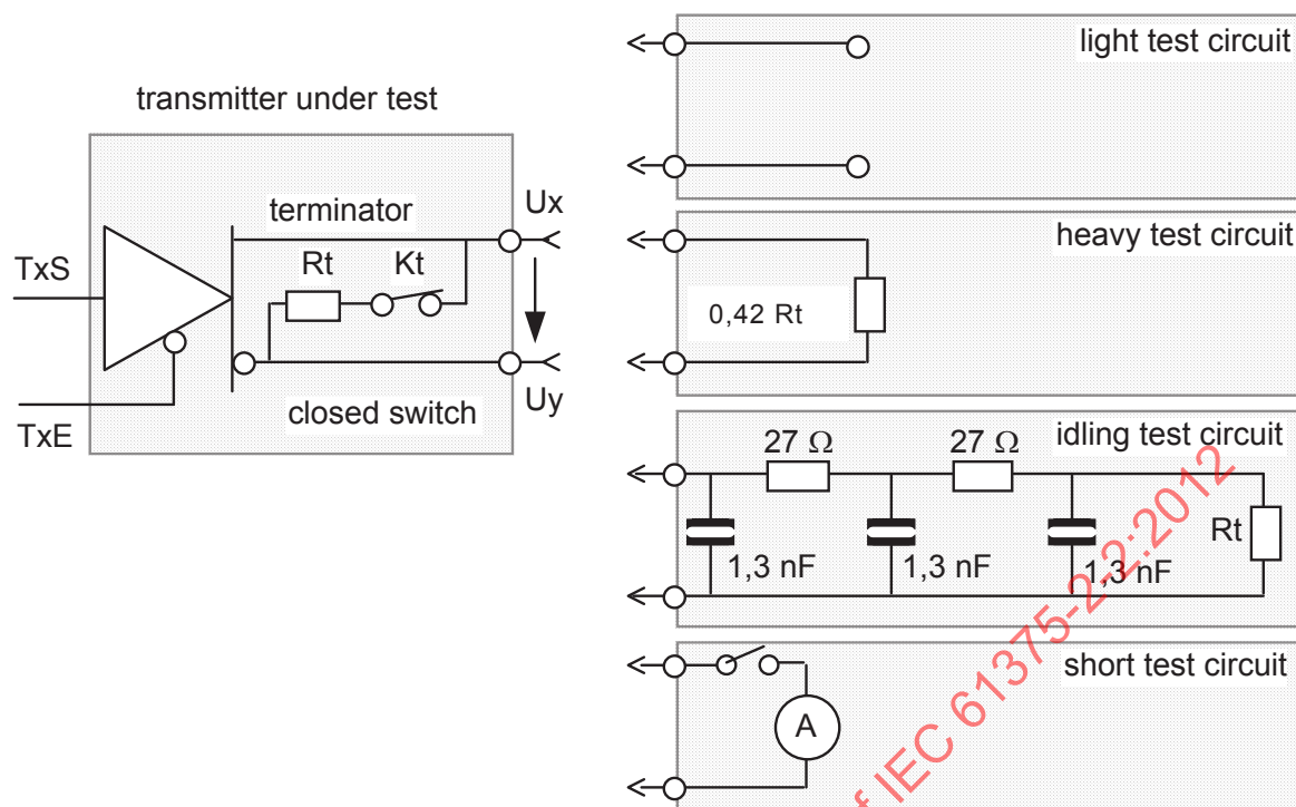
Figure 8 – Transmitter fixtures
