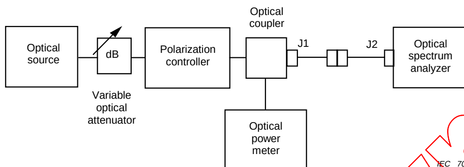
Figure 1a - Input signal power measurement
