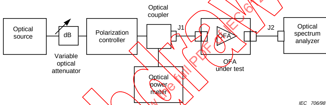
Figure 1b - Output signal power measurement
