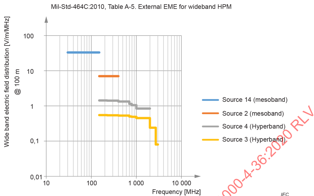
Figure B.10 – Wideband (mesoband and hyperband) EME derived from [B.17]
