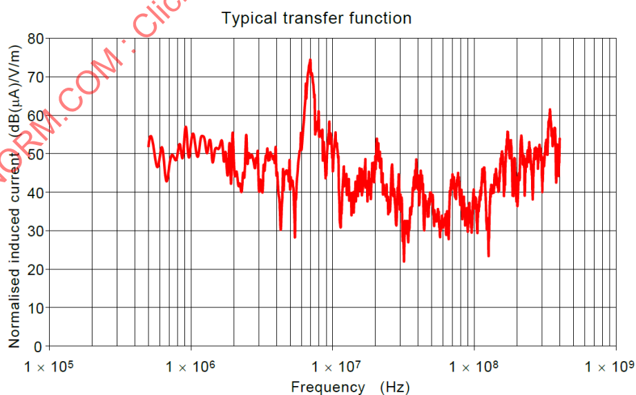
Figure E.3 – Typical LLSC magnitude-only transfer function
