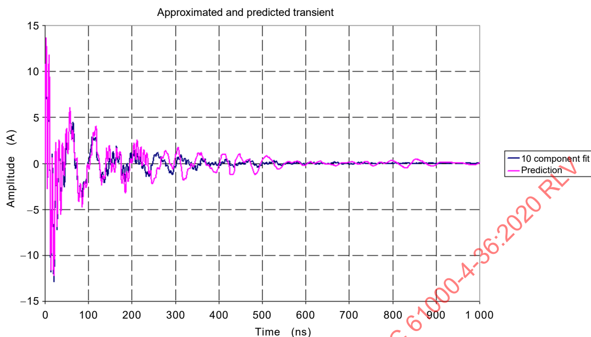
Figure E.10 – Approximated and predicted transient
