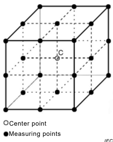
Figure I.1 – Example of the measurement points for the validation
