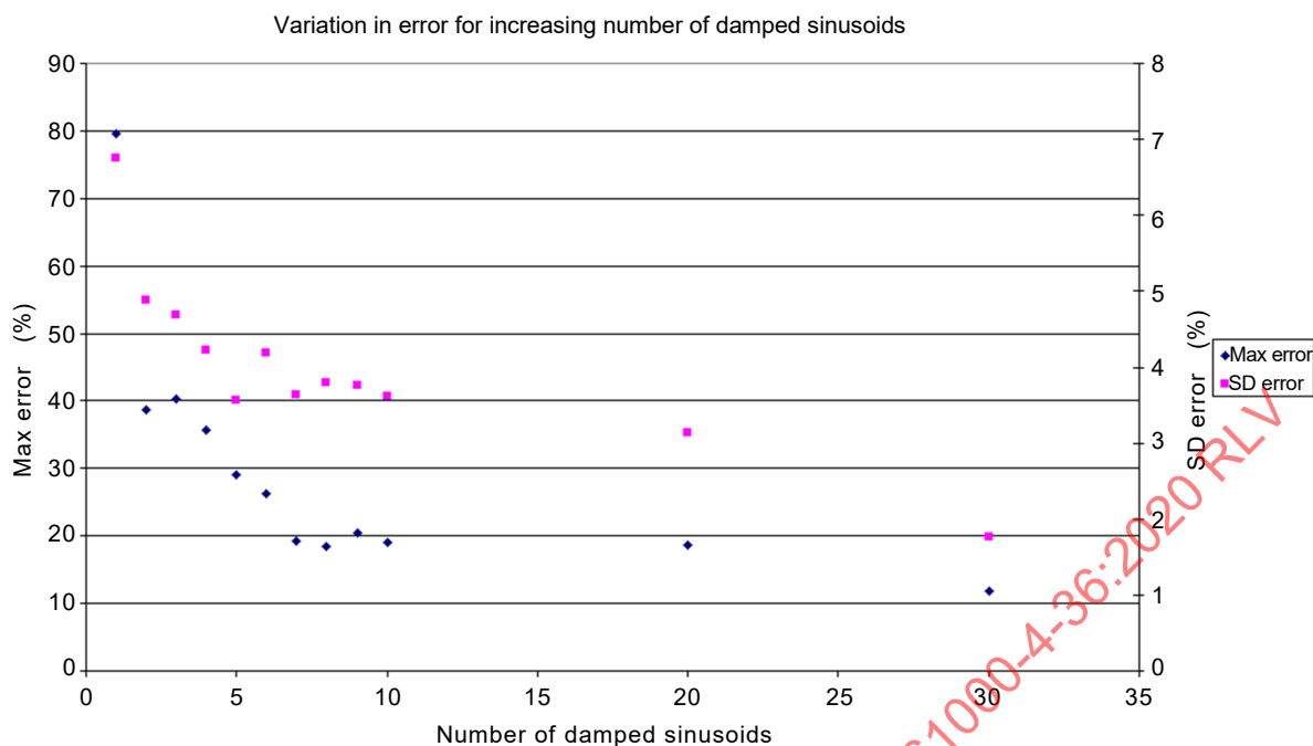
Figure E.13 – Variation in error for an increasing number of damped sinusoids
