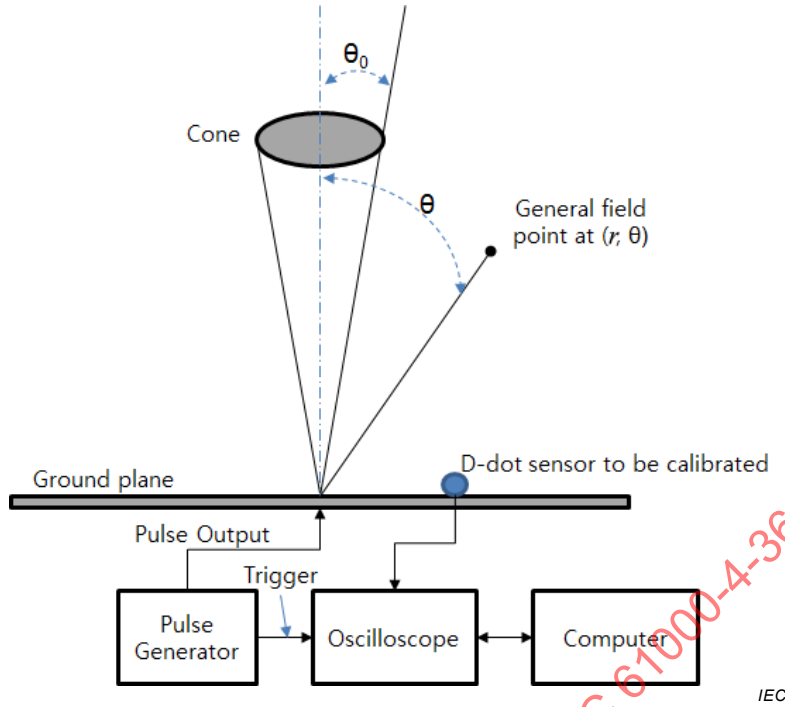
Figure I.3 – Cone and ground plane sensor calibration set-up
