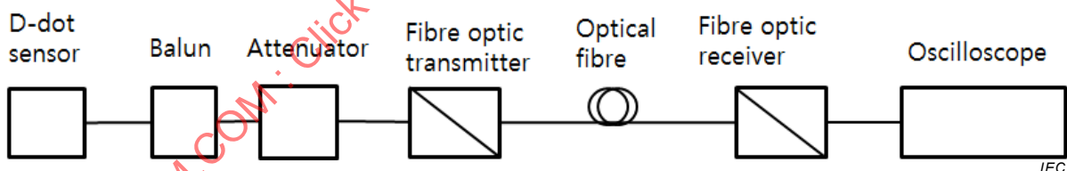
Figure H.1 – Measurement chain for field uniformity assessment and transient responses
