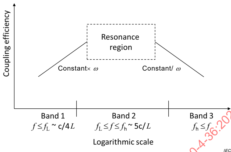
Figure C.2 – Cable coupling and resonance region
