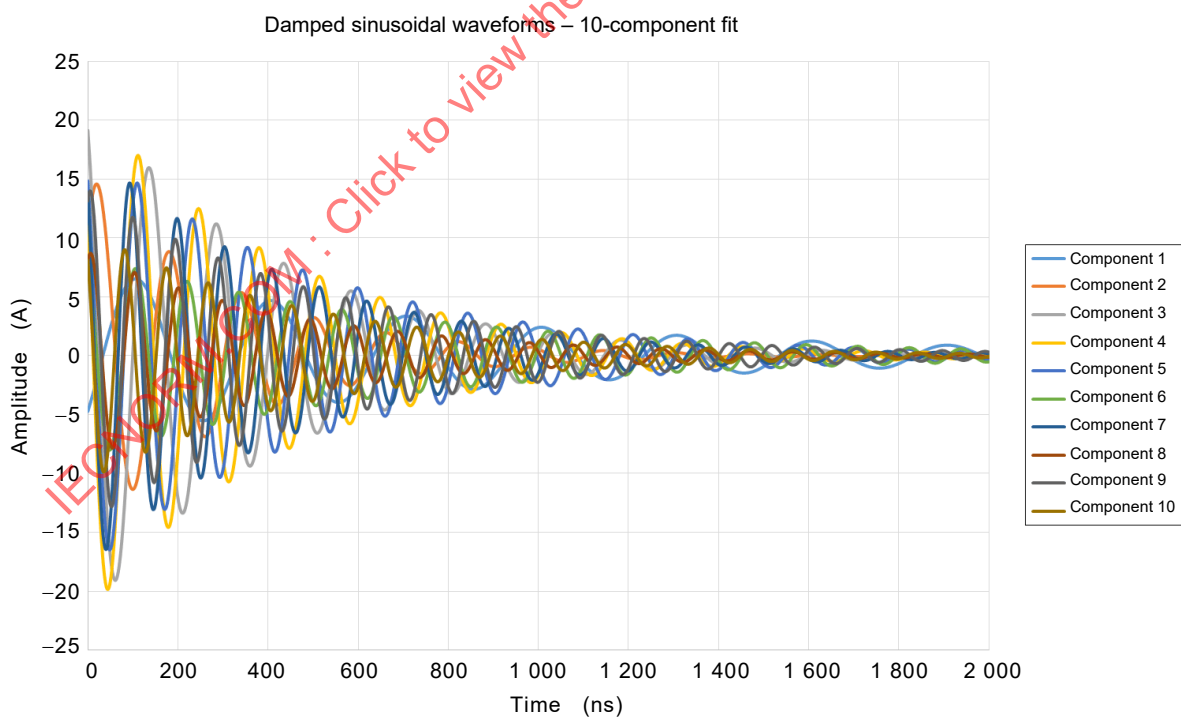
Figure E.9 – Damped sinusoidal waveforms – Ten-component fit
