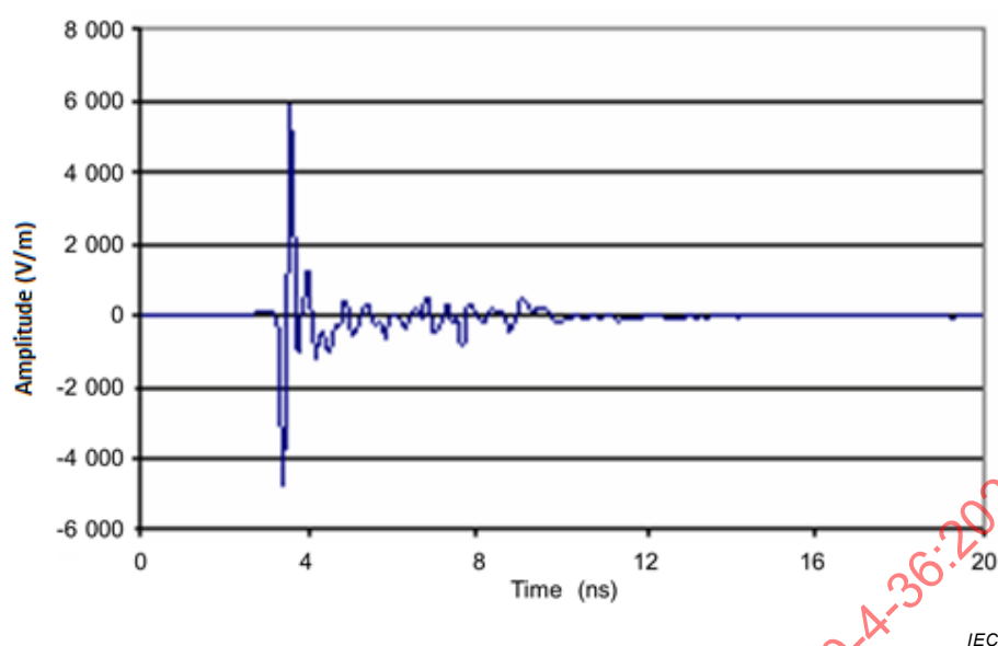
Figure 4 – Example of hyperband waveform
