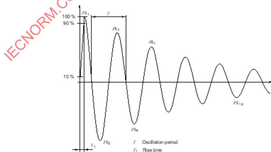
Figure 7 – Waveform of the damped oscillatory wave (open circuit voltage)
