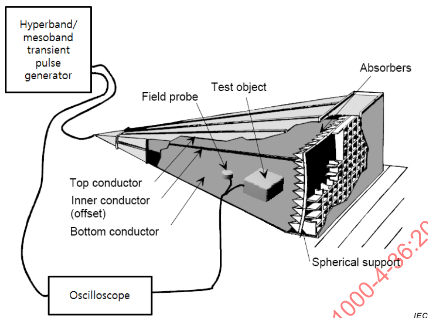
Figure H.5 – Example of test set-up in GTEM waveguide
