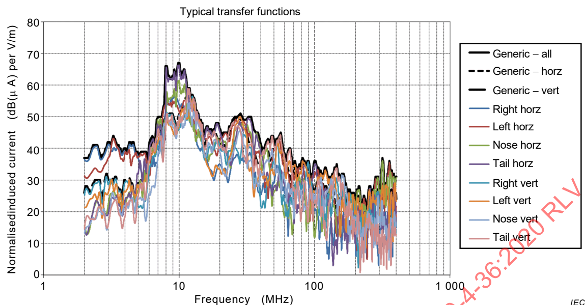
Figure F.5 – Example of transfer functions and worst-case envelope
