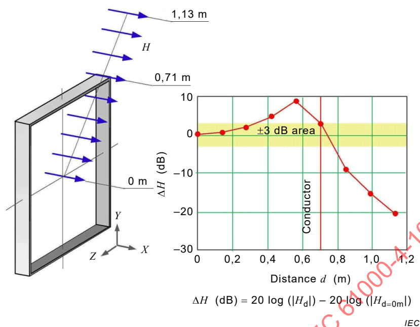
Figure E.5 – H_x -field along the diagonal in dB for the 1 m × 1 m standard induction coil
