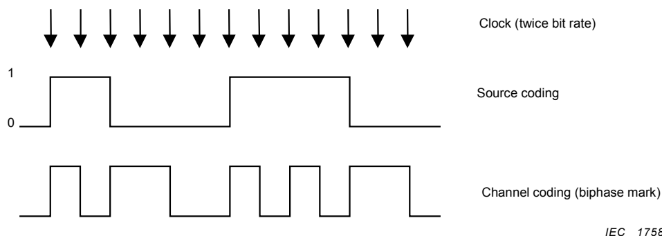
Figure 3 – Channel coding
