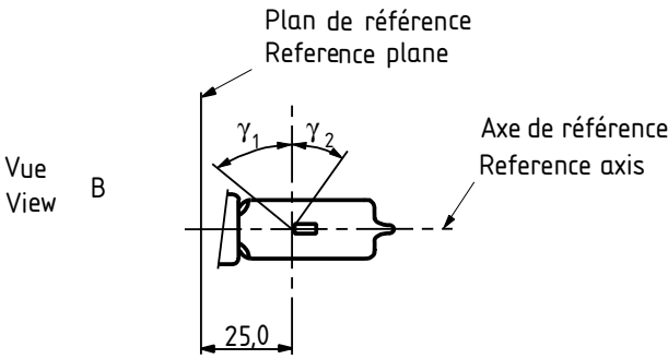
Figure 3 - Zone exempte de distorsion 5) Distortion-free area 5)
