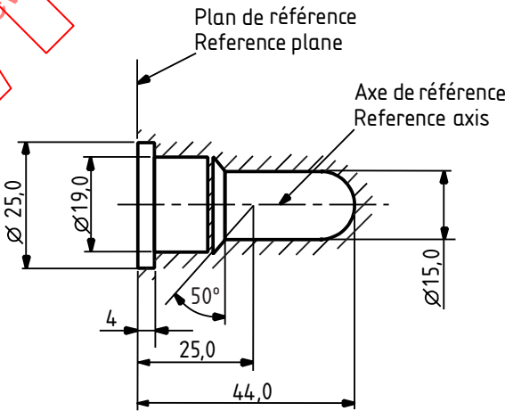
Figure 2 - Encombrement maximal de la lampe Maximum lamp outline 3)
