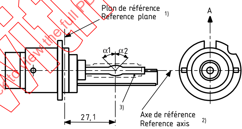
Figure 2 - Catégorie D2S; Type à broche; Culot P32d-2 Category D2S; Type with connector; Cap P32d-2
